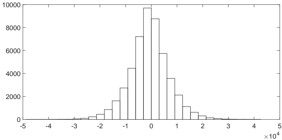
(b) Histogram of the implementation cost for the optimal trading strategies.
