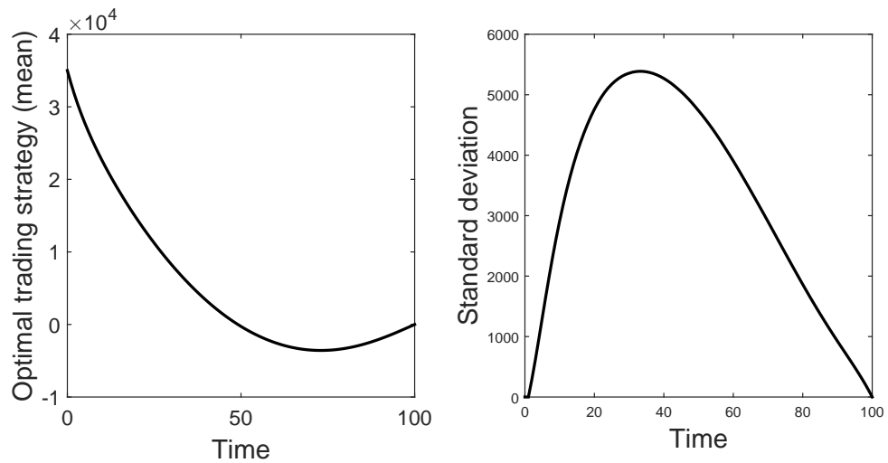
(a) Average and standard deviation of the optimal trading strategies with parameters given by Tables 1 when short selling is allowed.
