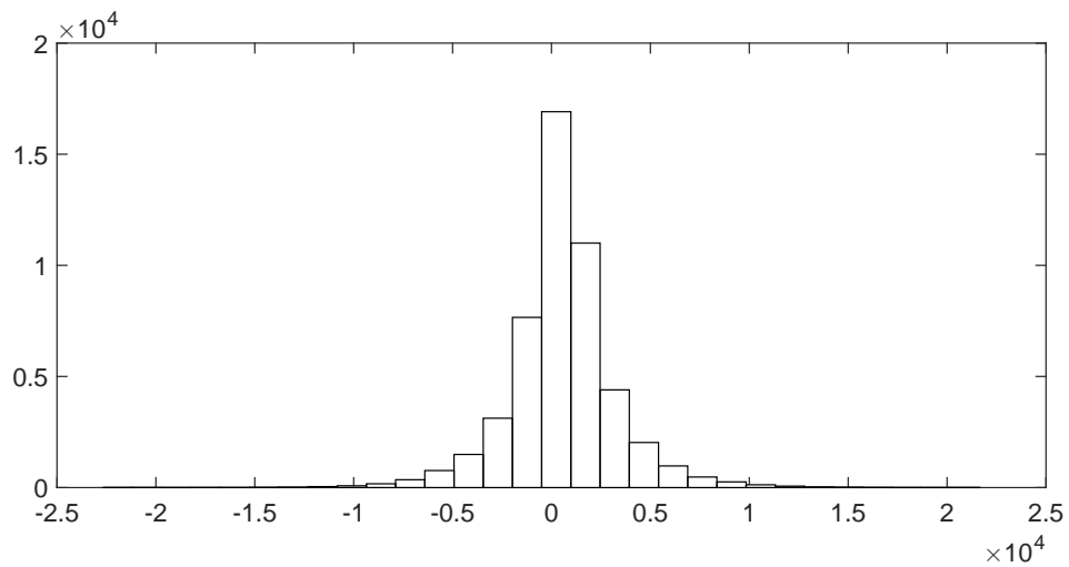
(b) Histogram of the implementation cost for the optimal trading strategies.
