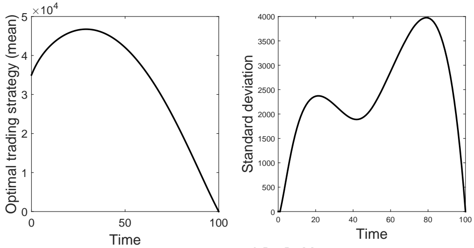
(a) Average and standard deviation of the optimal trading strategies with parameters given by Tables 1.
