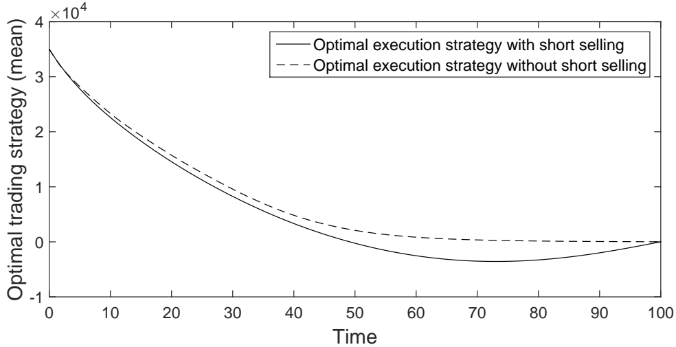
Figure 4: Comparison between optimal trading strategies when short selling is allowed and when it is denied.
