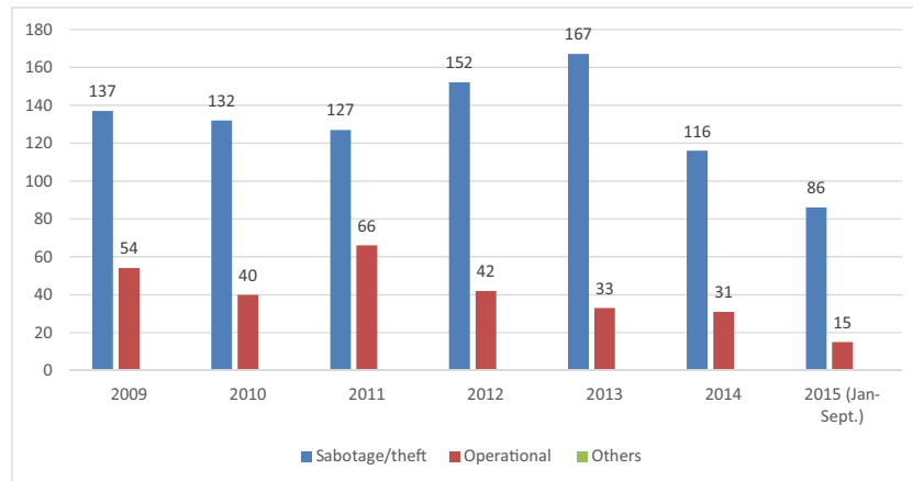
Figure 1. Number of oil spills/year (Shell, n.d.).
